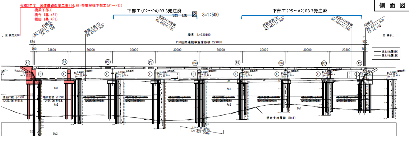
側面図(3-3)
